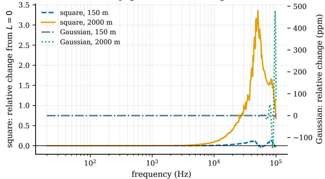
d Propagation-induced change
