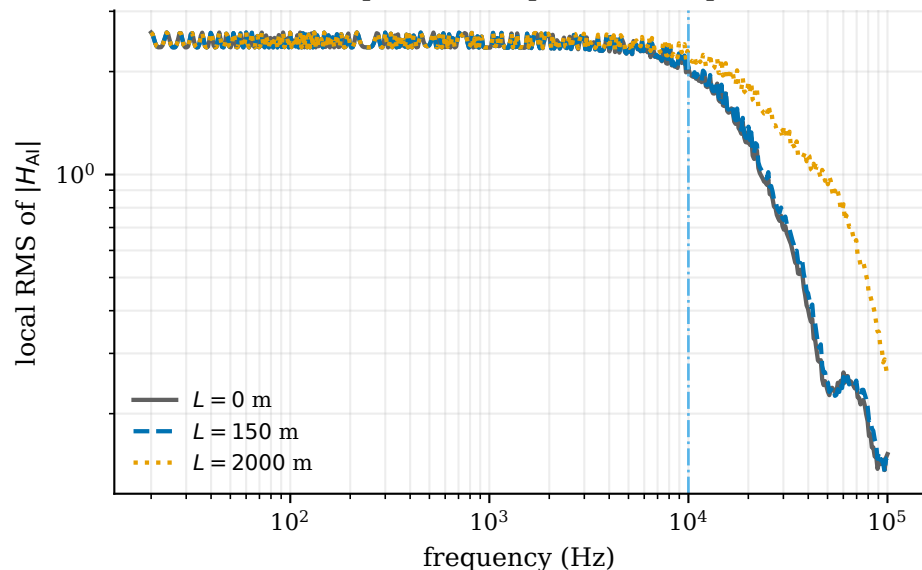
d Propagation-induced change
