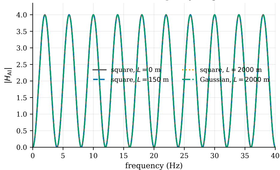
c Gaussian finite-pulse envelope
